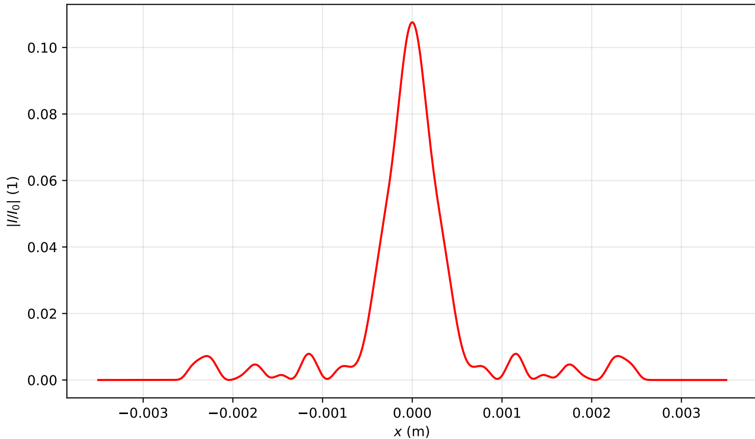
Intensity profile I(x, y = 0, z = 3.503)/I_0 , P_{in}=9.0P_{cr} , artificial time
